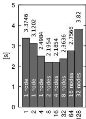
Pi approximated with 10,000,000 points (Mean Time of 5 Tests)
